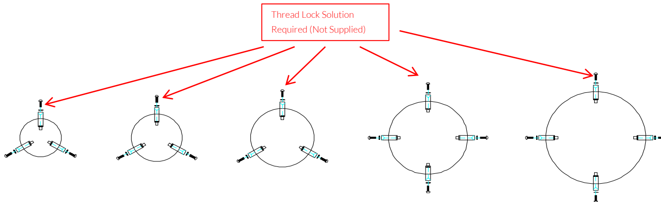
PPRASA PLAN
